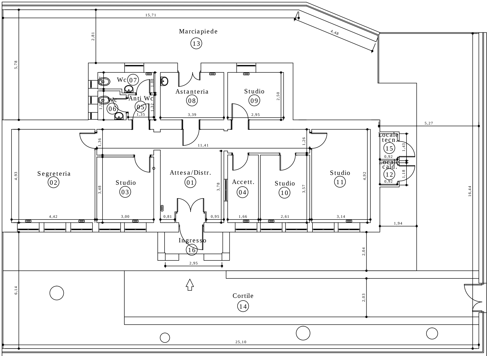
PIANO TERRA
